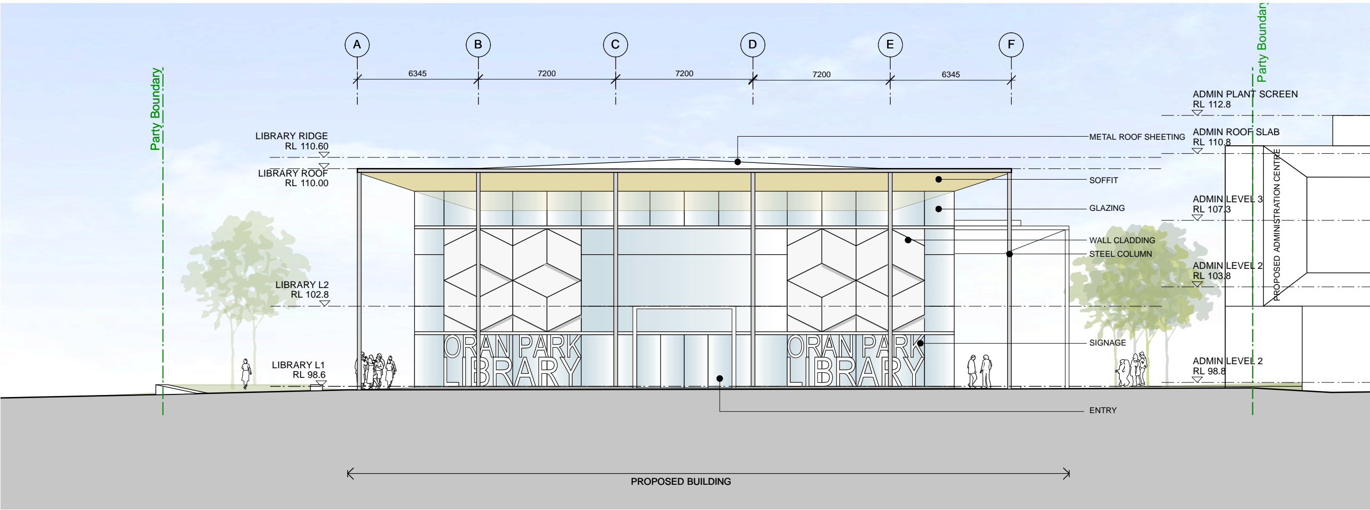
WEST ELEVATION- BUILDING ENVELOPE
