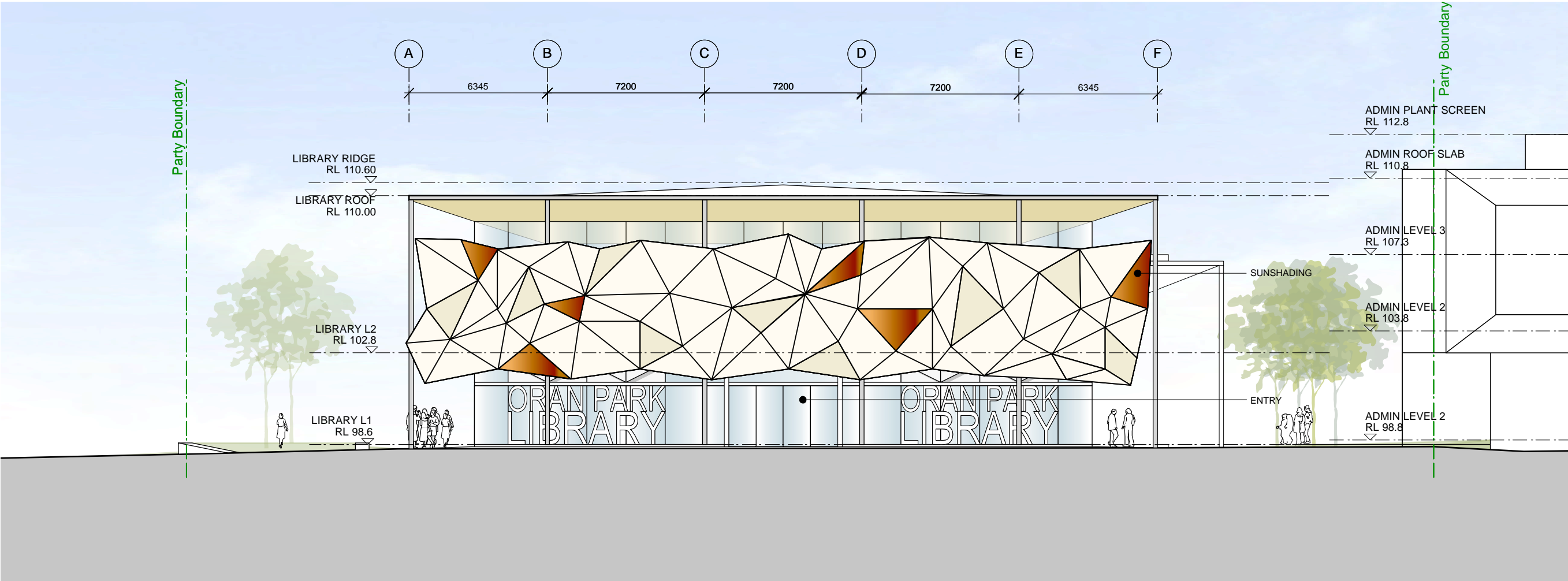
WEST ELEVATION - SUNSHADE
