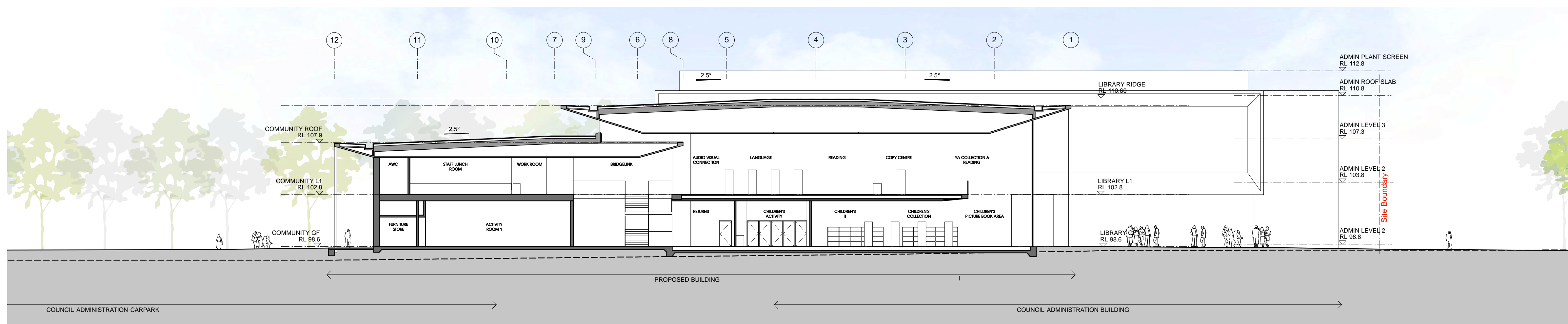
SECTION C
