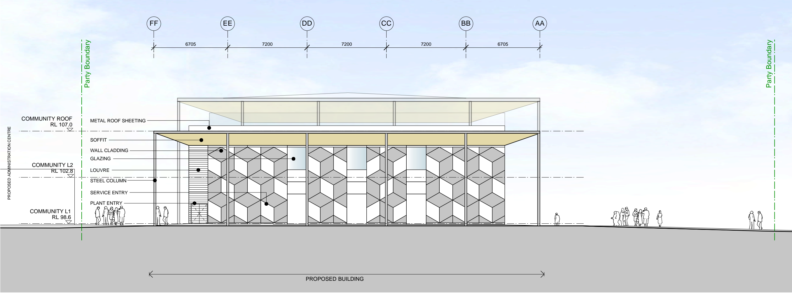
EAST ELEVATION
