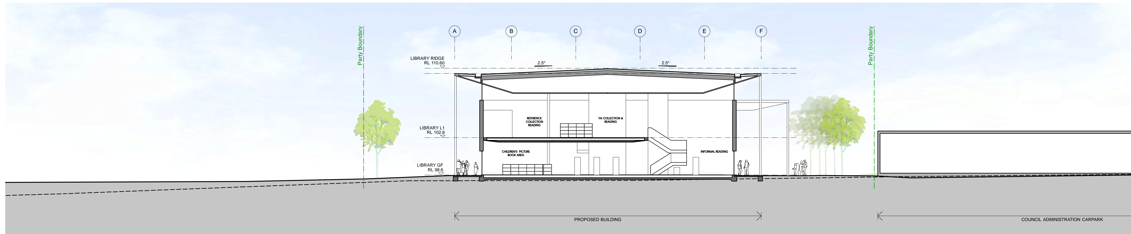
SECTION A | Library
